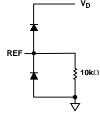
Figure 10. Reference Inputs
