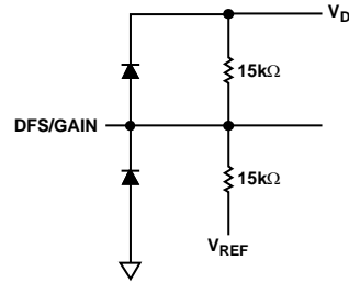
Figure 13. DFS/Gain Input
