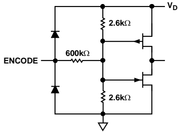
Figure 7. Encode Inputs
